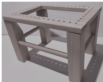
HAND CANING STOOL KIT
